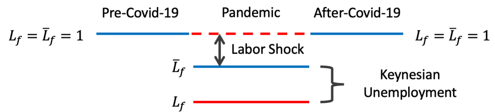
Figure 11. Schematic of the labor shock
