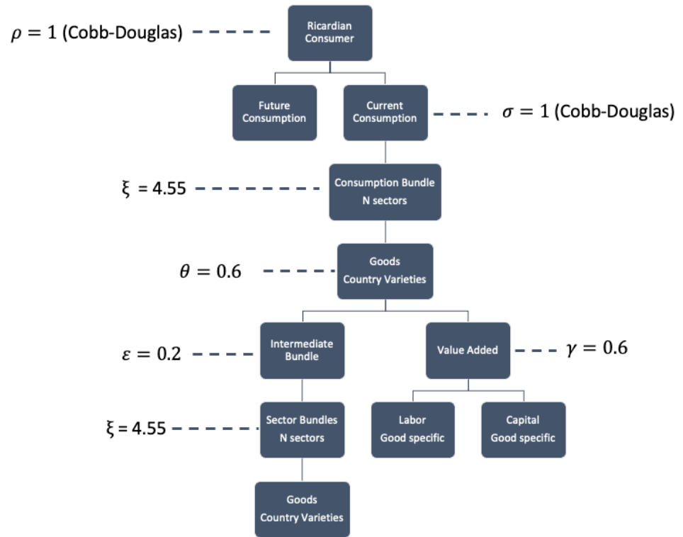
Figure 21. Schematic of the model.
