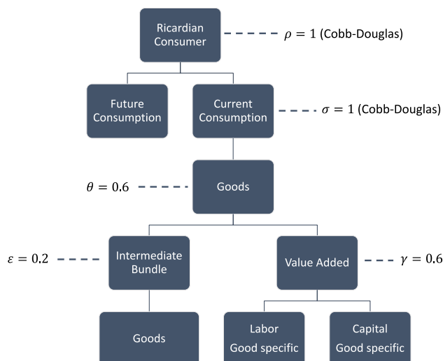
Figure 14. Schematic of the model
